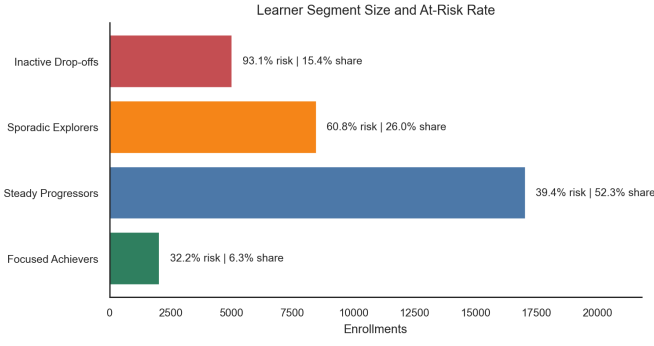
Fig. 3. Learner segment size and at-risk rate.
