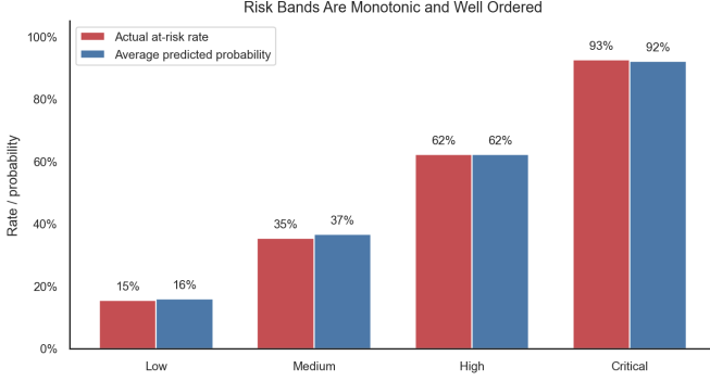
Fig. 5. Actual at-risk rate and average predicted probability by risk band.
