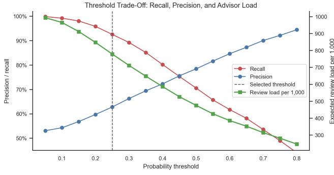
Fig. 7. Threshold trade-off between recall, precision, and expected advisor review load.
