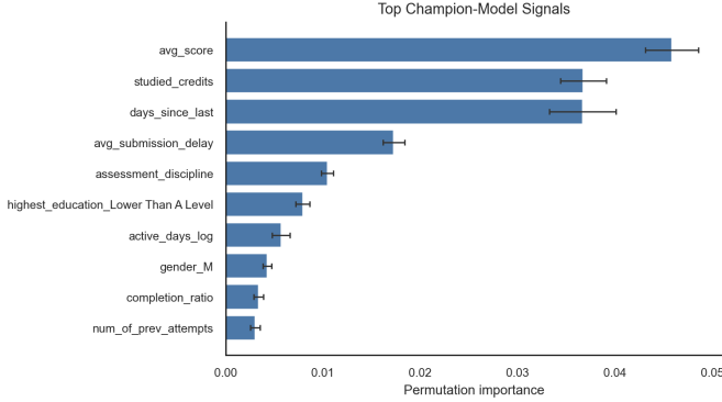
Fig. 6. Top champion-model signals by permutation importance.
