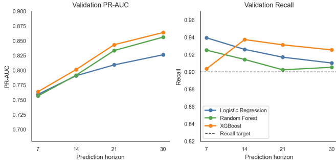
Fig. 4. Validation PR-AUC and recall across model families and prediction horizons.
